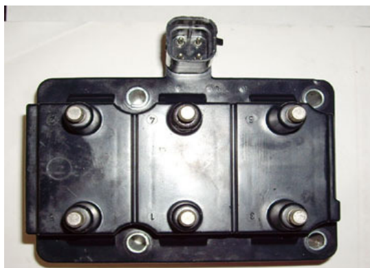
OEM: 5233140 Fit: GM
